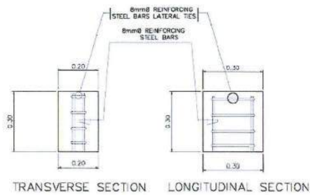
WHEEL GUARD DETAIL NTS
